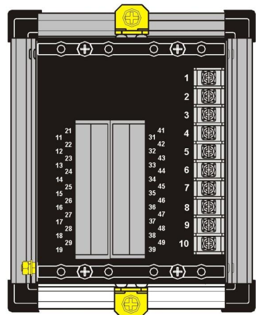
TERMINAL CONNECTION
