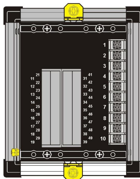
TERMINAL CONNECTION
